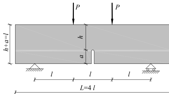
Figure 9-3 – Four point bending test on notched specimen.
